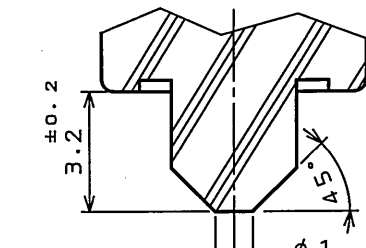
SECT. D-D (SCALE 5:1)
