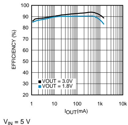
Figure 2. Efficiency of Buck 2
