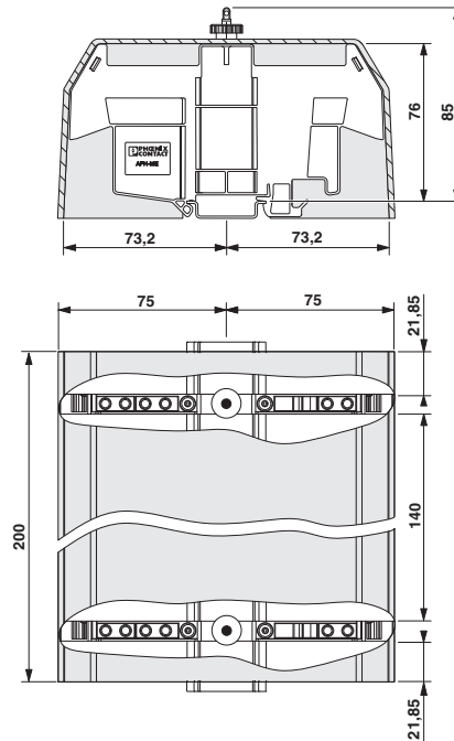
Dimensional drawing
