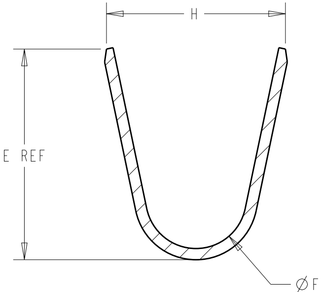
SECTION G-G
