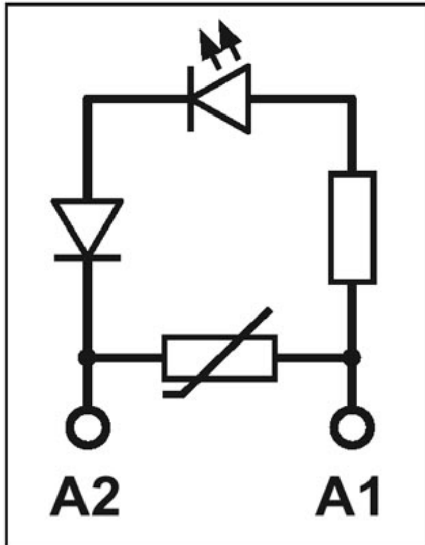
Circuit diagram
