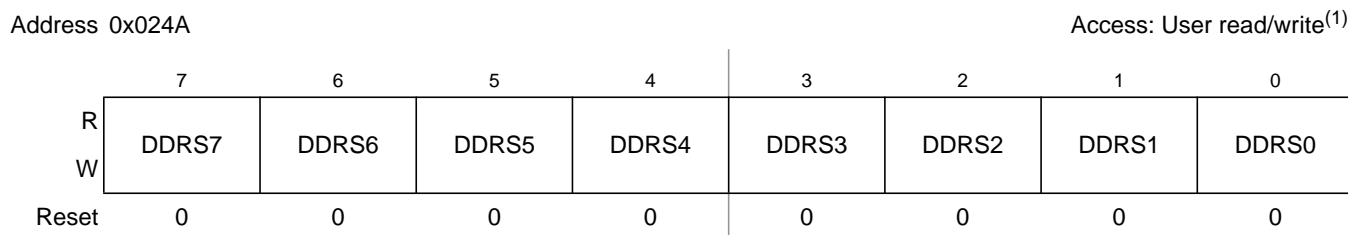
Figure 19-29. Port S Data Direction Register (DDRS)
