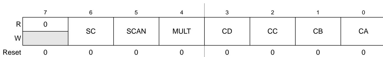
Figure 24-8. ATD Control Register 5 (ATDCTL5)
