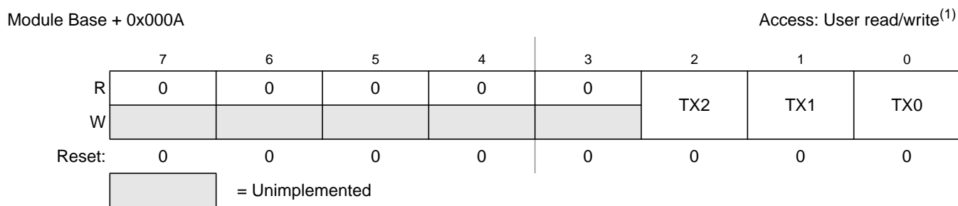
Figure 21-14. MSCAN Transmit Buffer Selection Register (CANTBSEL)
