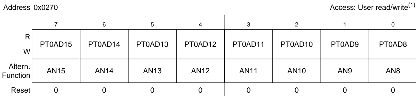
Figure 19-67. Port AD Data Register 0 (PT0AD)
