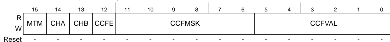
Figure 13-97. Message Buffer Cycle Counter Filter Registers (MBCCFRn)
