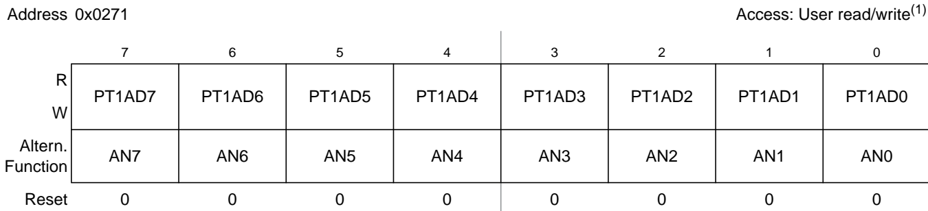
Figure 19-68. Port AD Data Register 1 (PT1AD)
