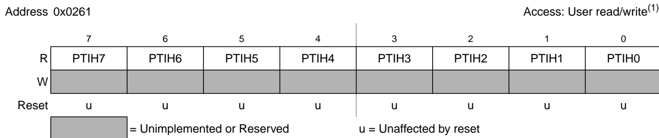
Figure 19-52. Port H Input Register (PTIH)
