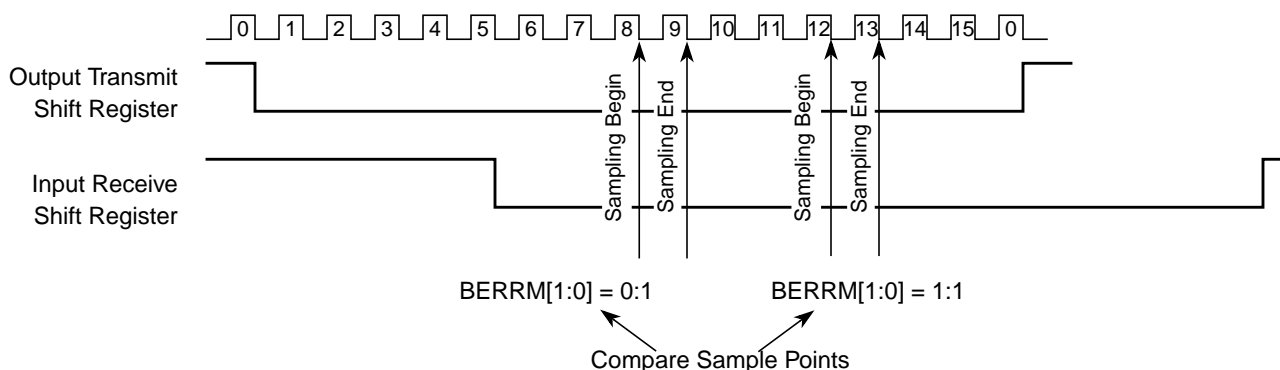
Figure 23-19. Timing Diagram Bit Error Detection
