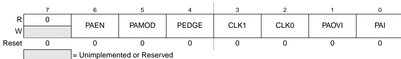
Figure 26-36. 16-Bit Pulse Accumulator Control Register (PACTL)
