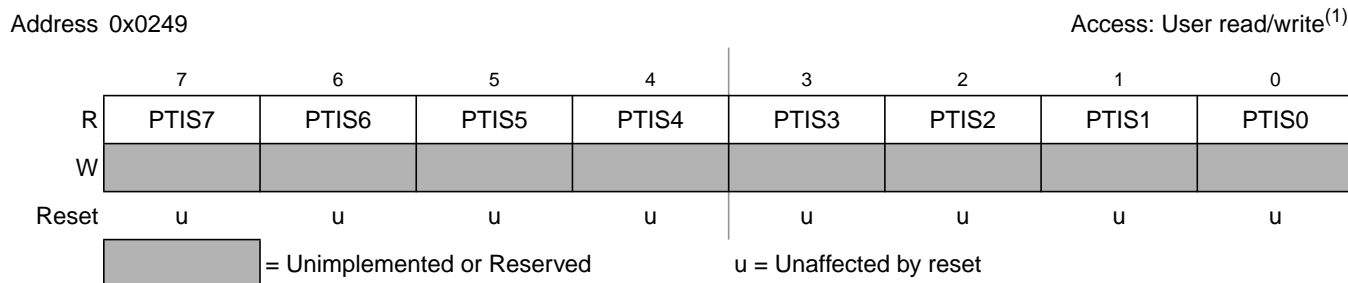
Figure 19-28. Port S Input Register (PTIS)
