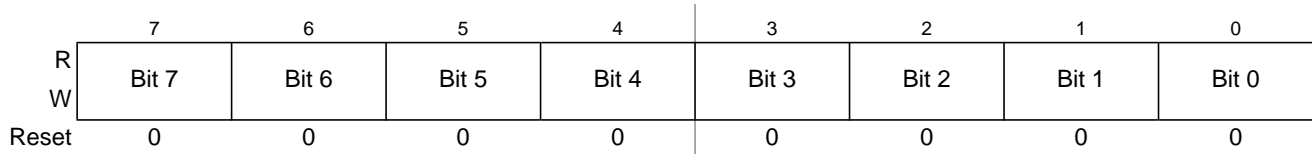
Figure 16-19. Debug Comparator Data Low Register (DBGXDL)
