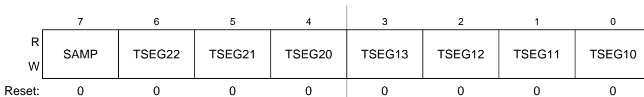
Figure 21-7. MSCAN Bus Timing Register 1 (CANBTR1)
