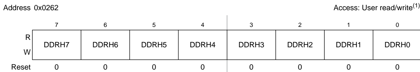
Figure 19-53. Port H Data Direction Register (DDRH)
