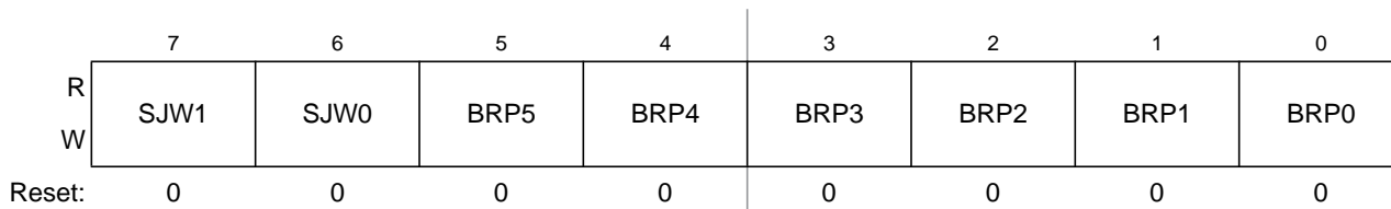
Figure 21-6. MSCAN Bus Timing Register 0 (CANBTR0)
