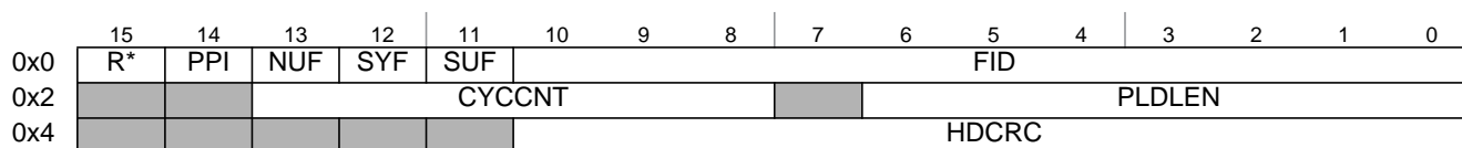
Figure 13-105. Frame Header Structure
