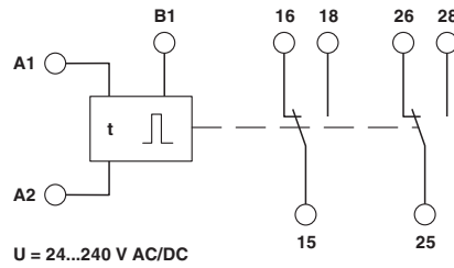
Block diagram
