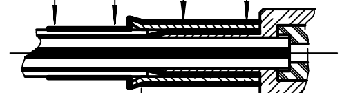
Crimping area
