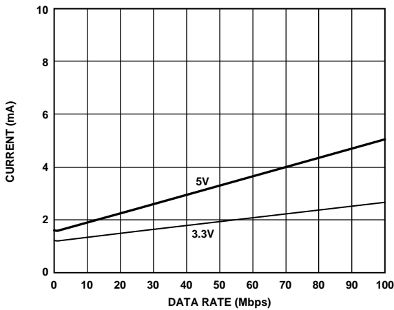
Figure 19. Typical Supply Current per Output Channel vs. Data Rate for 5 V and 3.3 V Operation (No Output Load)
