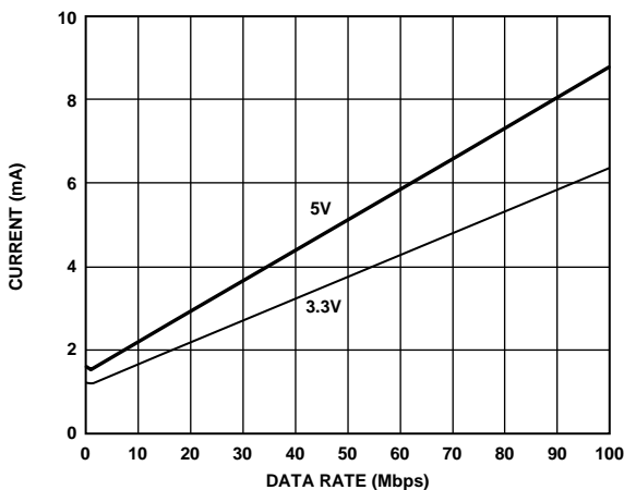
Figure 20. Typical Supply Current per Output Channel vs. Data Rate for 5 V and 3.3 V Operation (15 pF Output Load)
