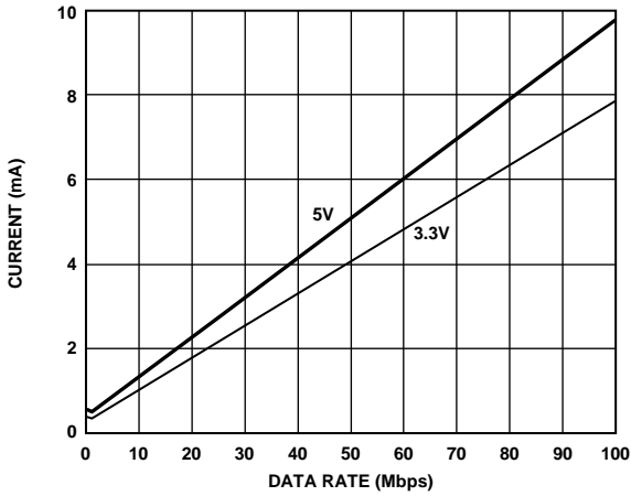
Figure 18. Typical Supply Current per Input Channel vs. Data Rate for 5 V and 3.3 V Operation (No Output Load)
