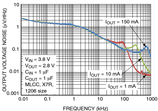
Figure 30. Output Voltage Noise Spectral Density for V_{OUT} = 2.8\text{ V} , C_{OUT} = 1\text{ }\mu\text{F}
