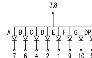
POLARITY DIAGRAM
