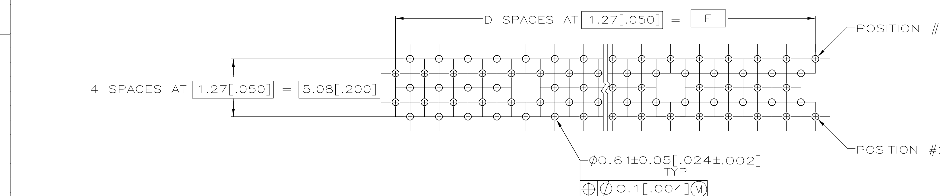
RECOMMENDED PC BOARD HOLE LAYOUT (VIEWED FROM CONNECTOR SIDE) SCALE 5:1
