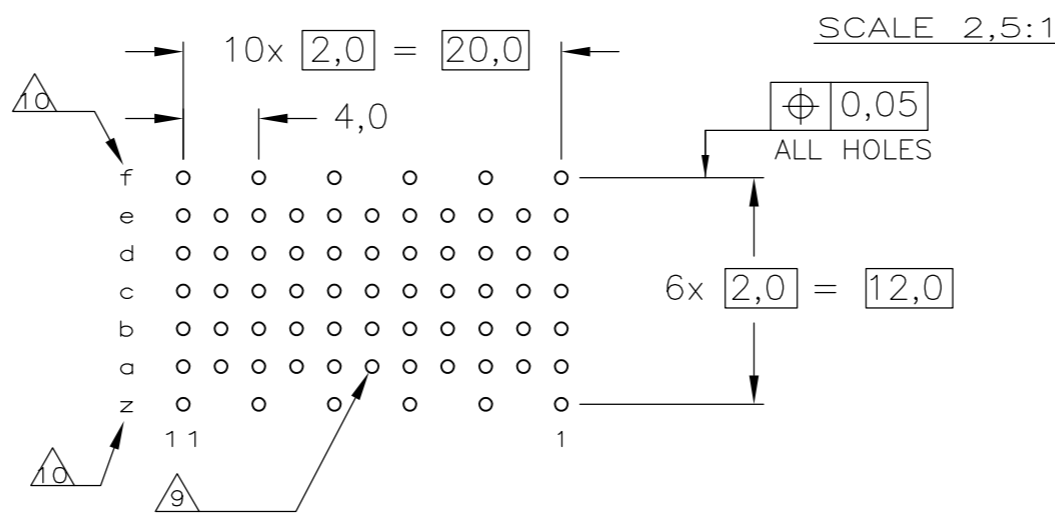
COMPONENT SIDE AS SHOWN RECOMMENDED PCB-HOLE LAY-OUT
