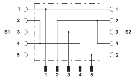
Contact assignment of the M12 T distributor
