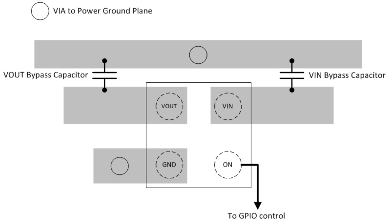
Figure 32. Layout Example
