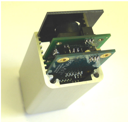
Motherboard, Two Daughterboards, and One Top Panel, partially inserted.
