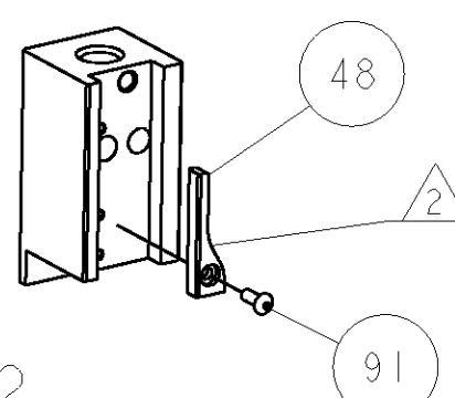
PRE-FEED 1 1/8 STROKE
