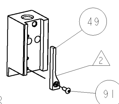
PRE-FEED 1 5/8 STROKE
