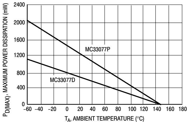
Figure 2. Maximum Power Dissipation versus Temperature
