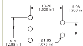
P.C. MOUNTING
