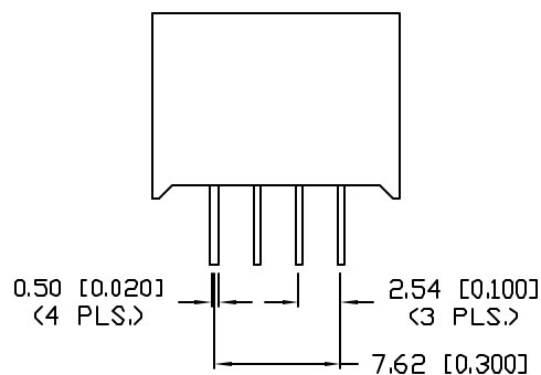
PIN OUT
