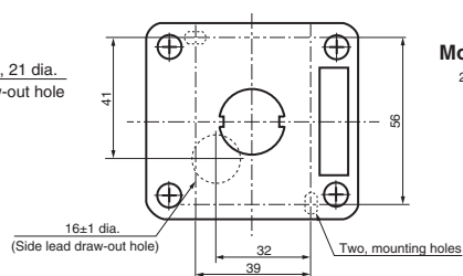
Cable Draw-out Hole (Top View)
