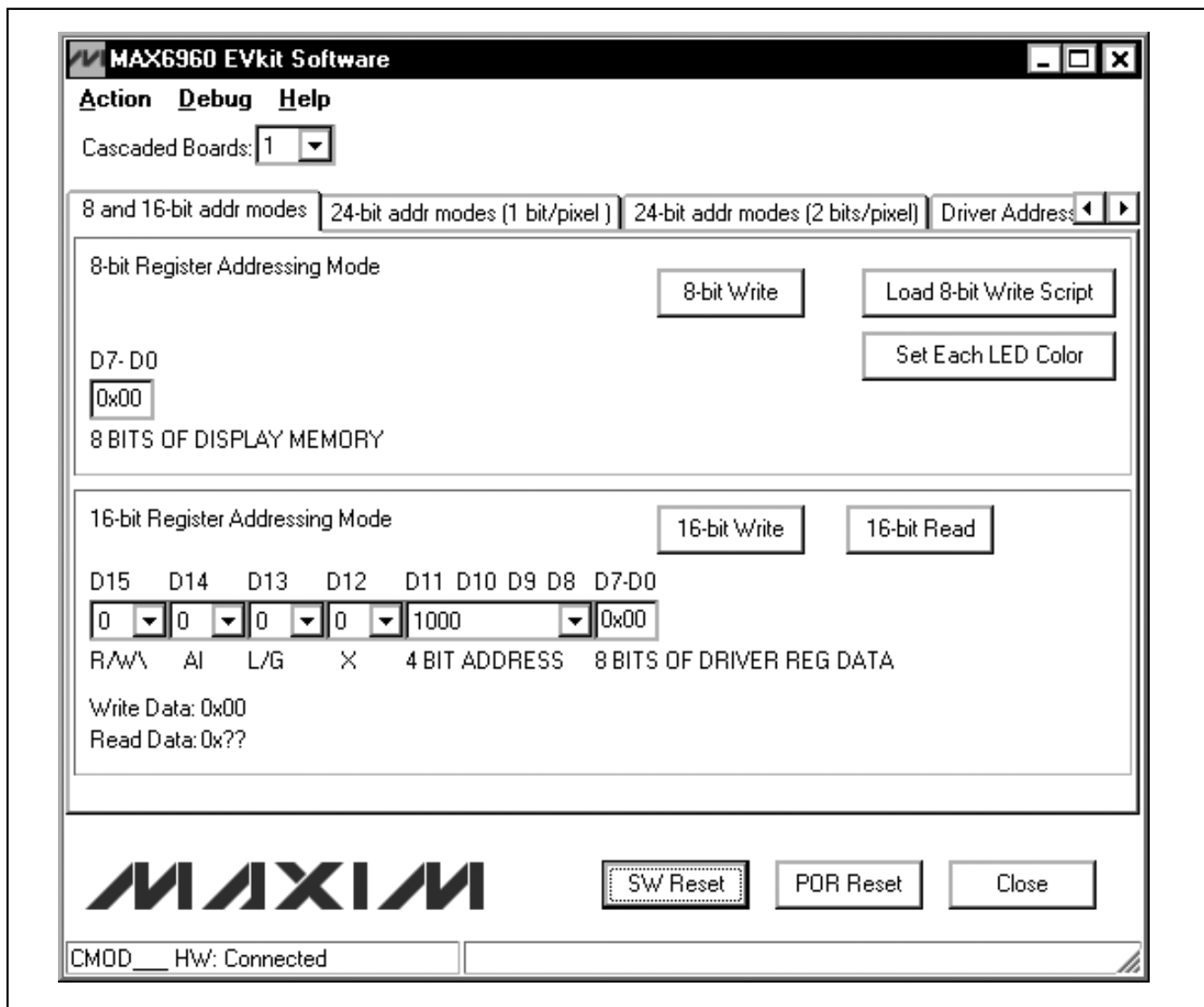
Figure 1. MAX6960 Evaluation Software Main Window
