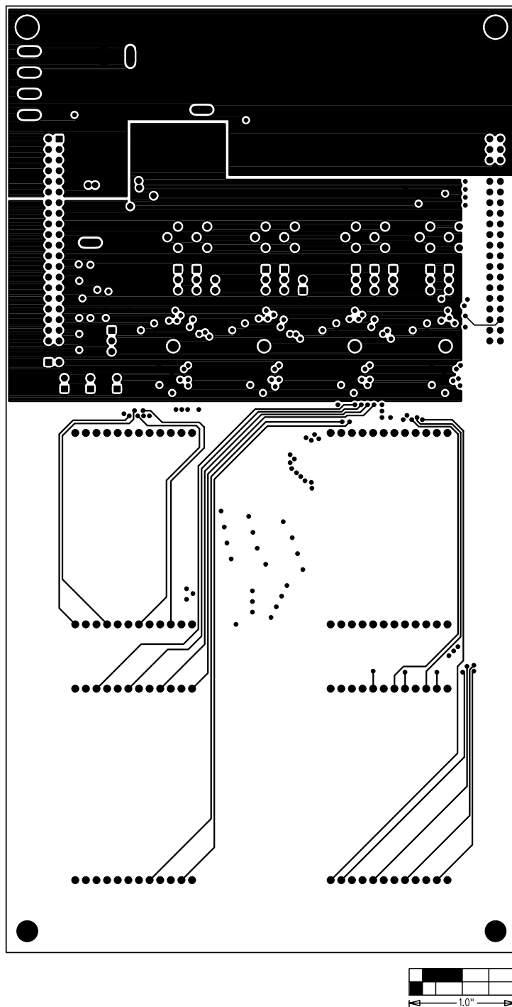
Figure 9. MAX6960 EV Kit PC Board Layout—Inner Layer 3 (VCC)
