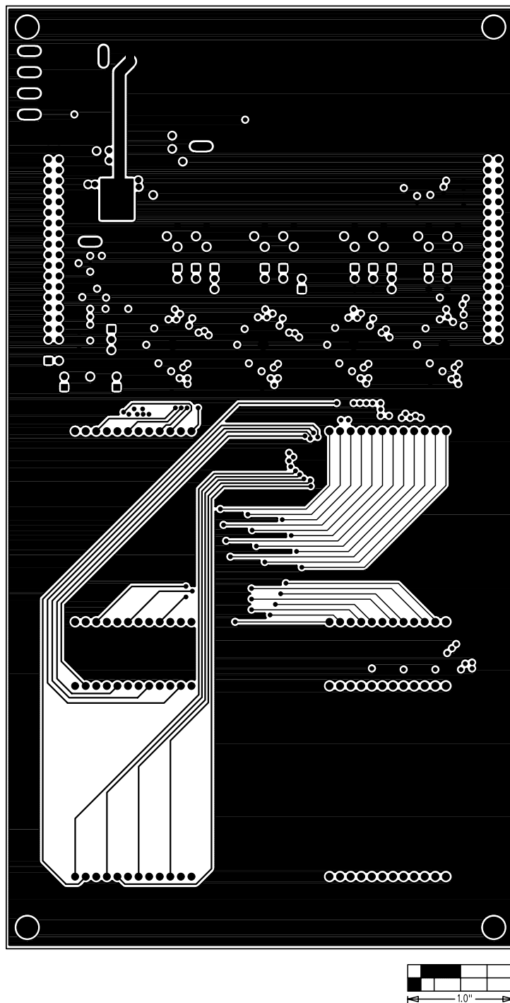
Figure 8. MAX6960 EV Kit PC Board Layout—Inner Layer 2 (GND)
