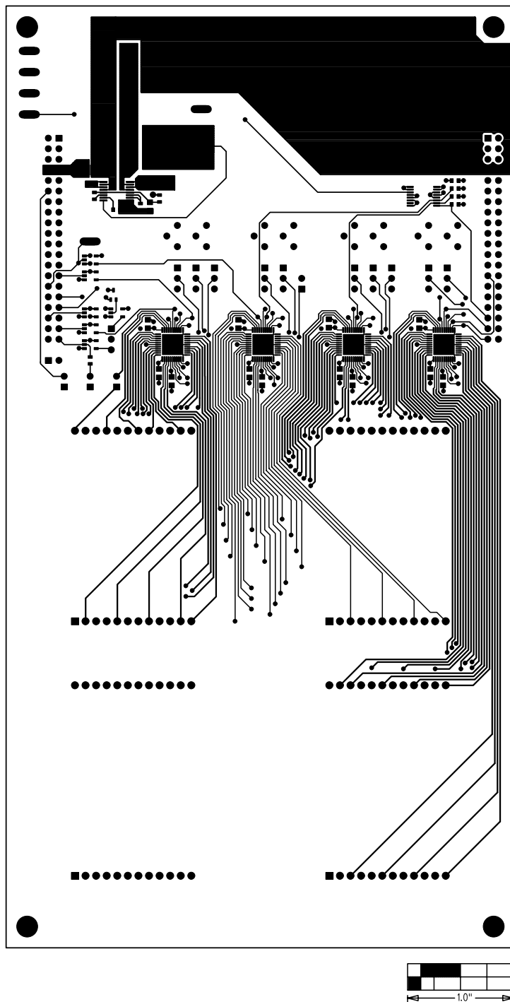
Figure 7. MAX6960 EV Kit PC Board Layout—Component Side
