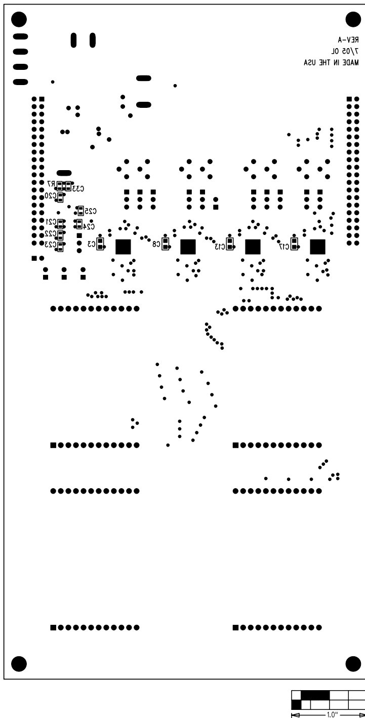
Figure 11. MAX6960 EV Kit Component Placement Guide—Solder Side
