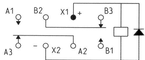
TERMINAL VIEW
