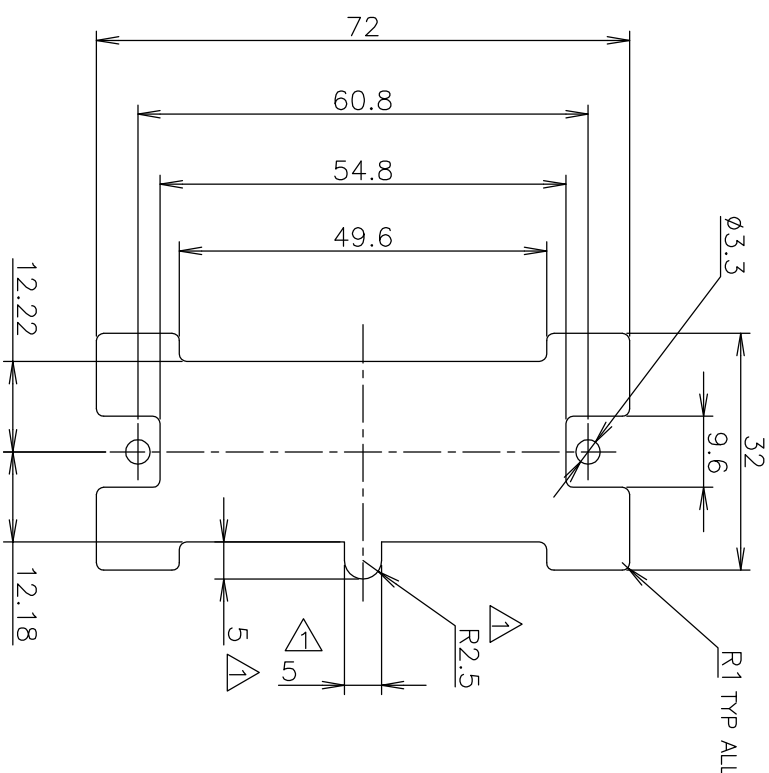
PANEL CUT DIMENSIONS (FRONT MOUNT)
