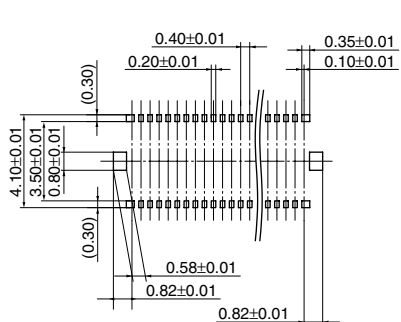
Recommended metal mask pattern
