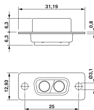
Dimensional drawing
