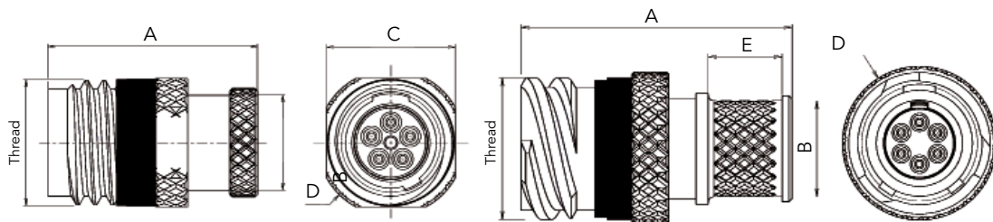
Shell size 3
