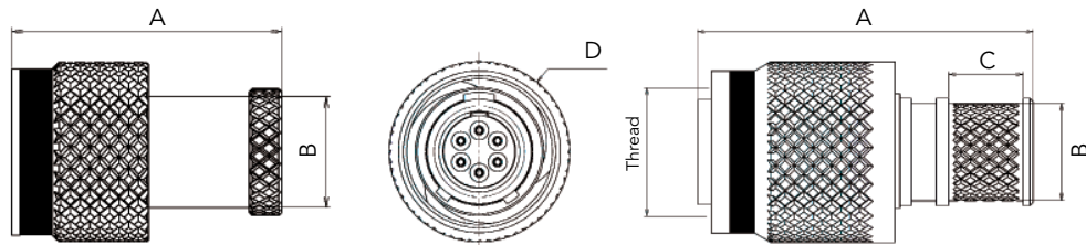
Shell size 3
