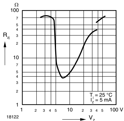
Fig. 7 - Dynamic Resistance vs. Zener Voltage
