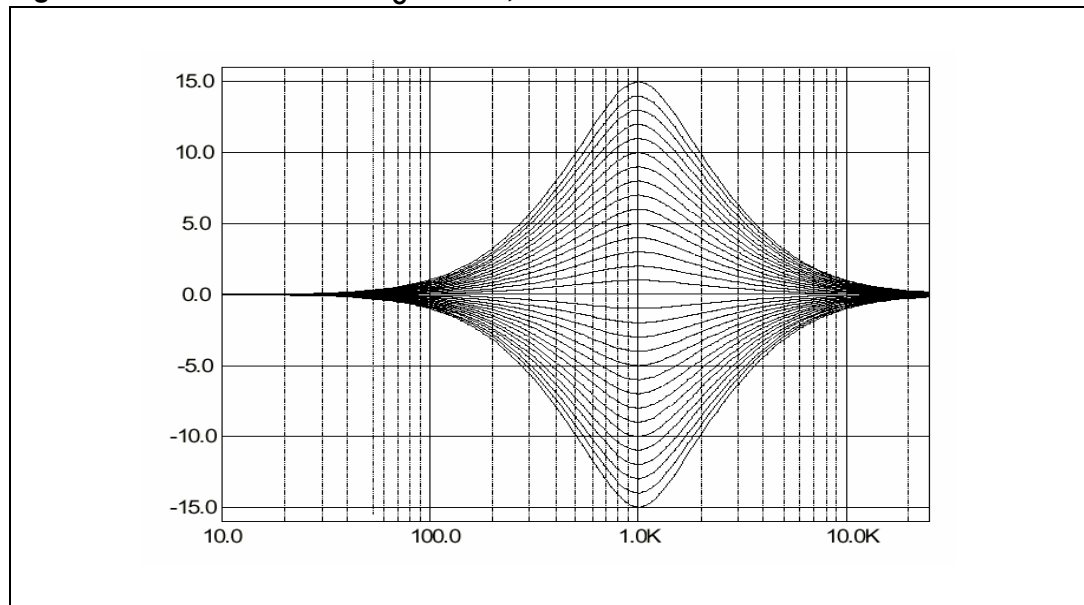
Figure 12. Middle control @ f_C = 1 \text{ kHz} , Q = 1
