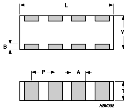
Fig. 2 Surface mounted multilayer ceramic capacitor dimension
