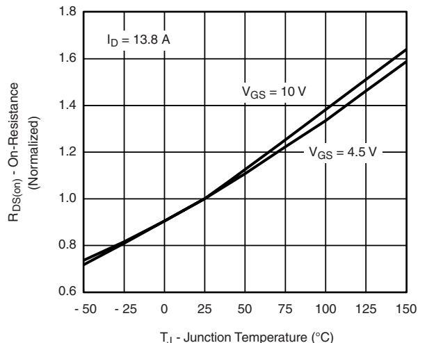
I_D = 13.8\text{ A} V_{GS} = 10\text{ V} V_{GS} = 4.5\text{ V} On-Resistance vs. Junction Temperature
