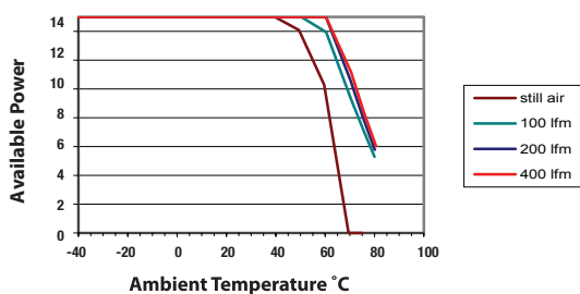
RUW15SL24HC
