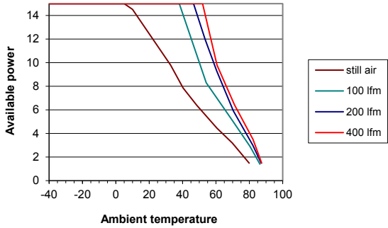
RUW15SL24C
