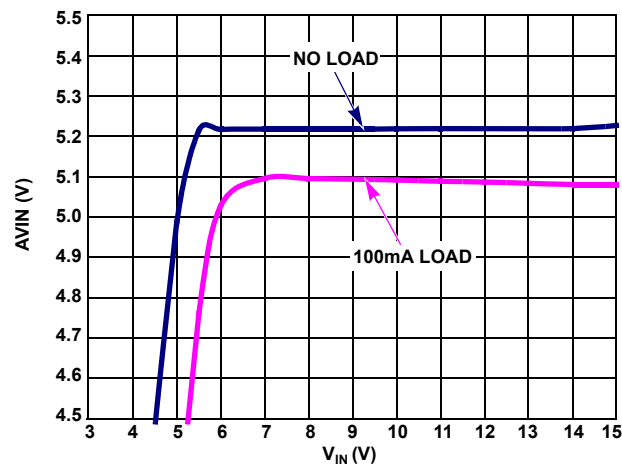
FIGURE 22. V_{AVIN} REGULATION vs V_{IN}
