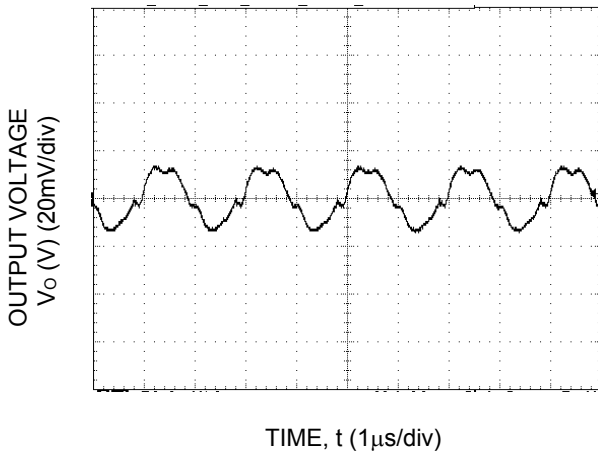
Fig-17. Typical output ripple and noise ( C_O=2x47\mu F ceramic, V_{IN} = 12V , I_o = I_{o,max} ).
