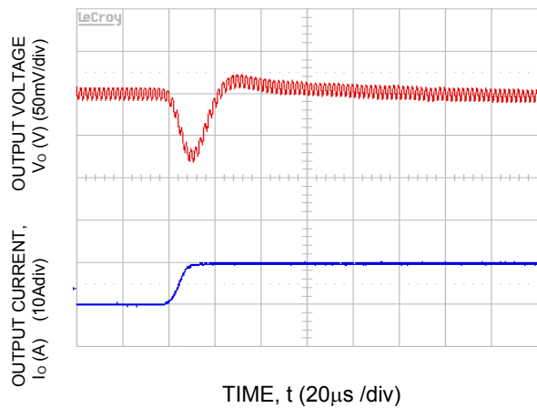
Fig-18. Transient Response to Dynamic Load Change from 50% to 100% at 12Vin, C_{out}= 8x47\mu F , C_{Tune}=1500pF & R_{Tune}=220ohms
