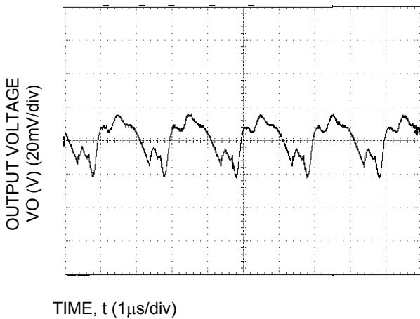
Fig-35. Typical output ripple and noise (C O =2x47µF ceramic, V IN = 12V, I o = I o,max ).
