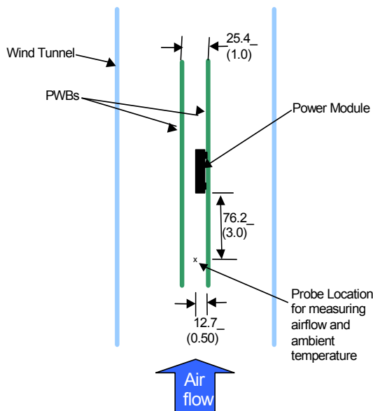
Fig-13: Thermal test set-up
