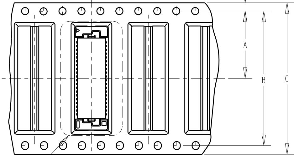
DETAIL B
